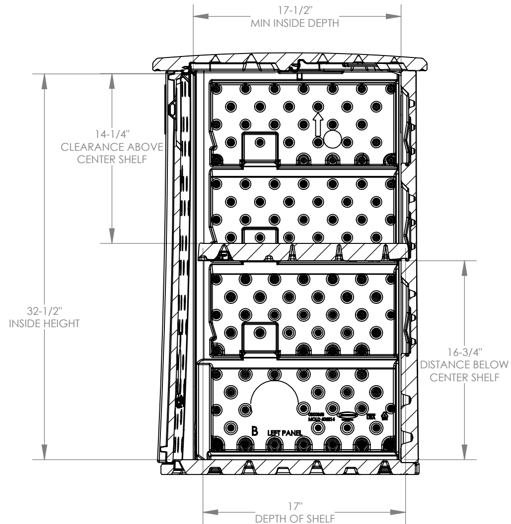
SIDE SECTION VIEW
